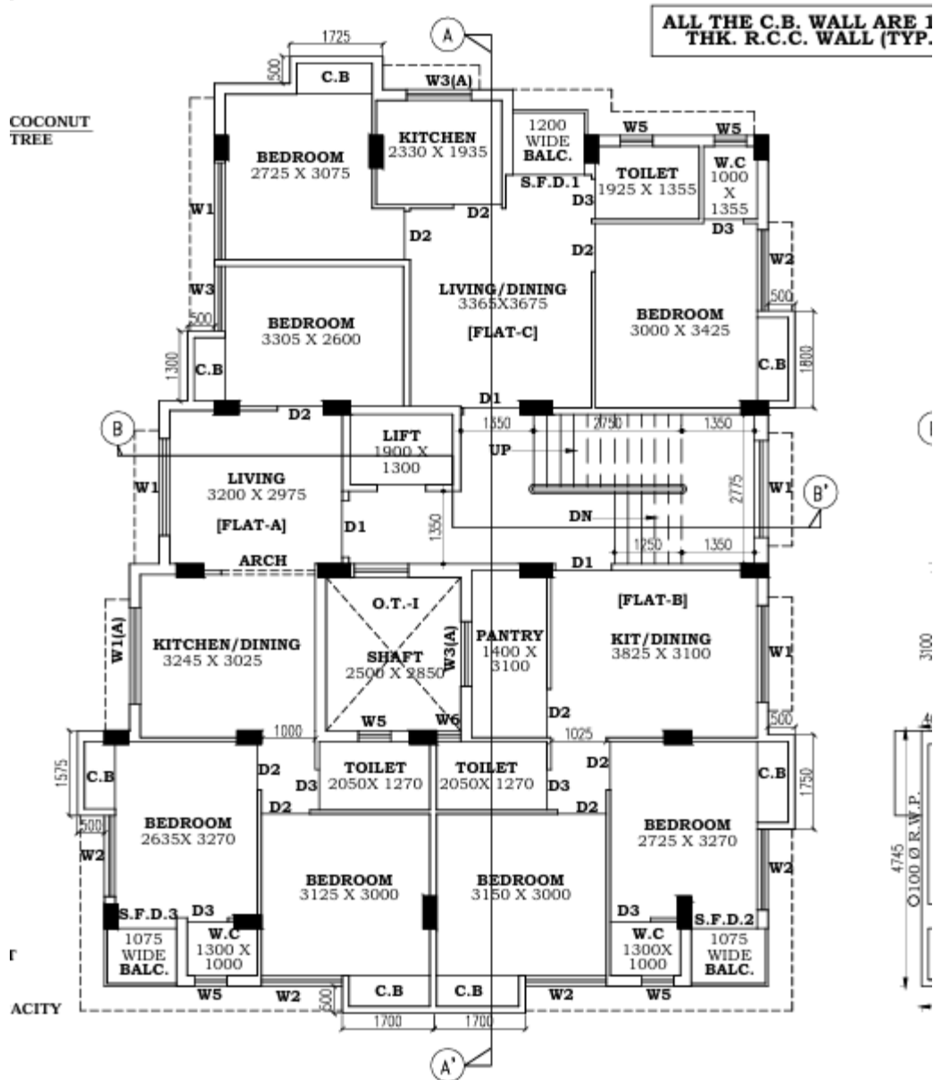
TYPICAL (1ST TO 4TH) FLOOR PLAN (SCALE: 1 : 100)
